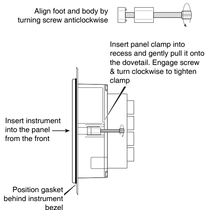
Fig 3 Installation of panel and mounting clamps
