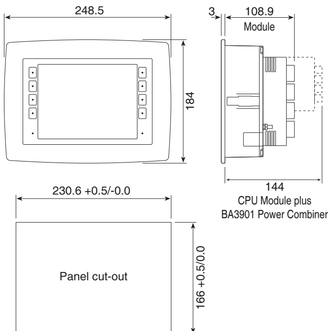
Fig 2 BA3101 dimensions including plug-in modules and panel cut-out
