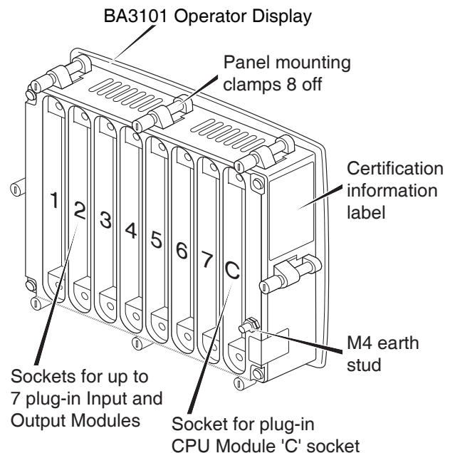
Fig 1 Rear view without plug-in modules
